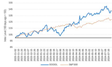
GOOGL vs S&P 500 (180 days) performance
