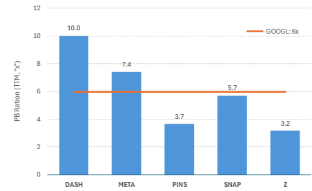
PB ratios
